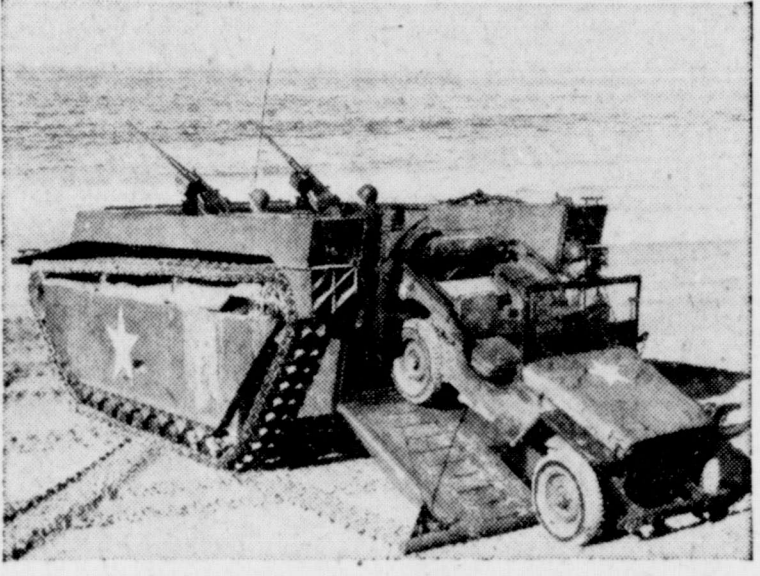
The "Water Buffalo" amphibious tractor, ace war weapon, is going to be de-horned and produced for peaceful purposes by its creator, Food Machinery Corporation. This armored and armed Water Buffalo is similar to the peace-time models except the armor and "horns" will come off and it will weigh less; carry more.
