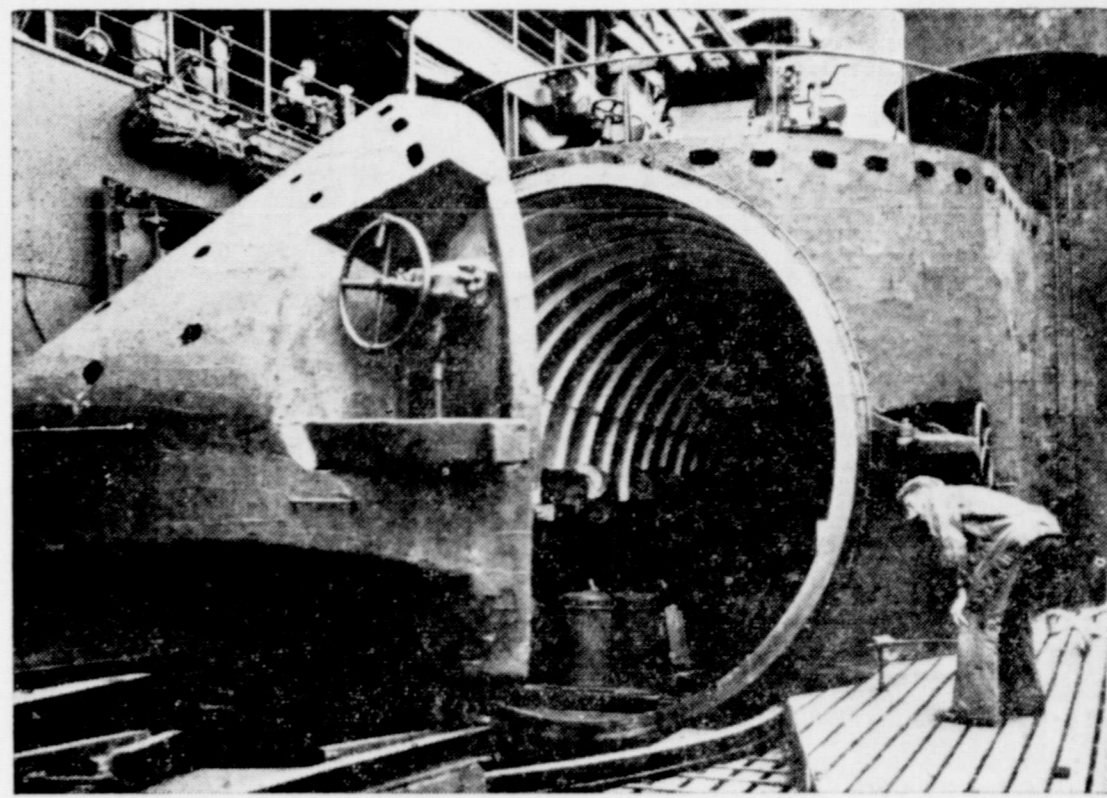
SUBMARINE AIR BASE—This is the "hangar" entrance of what is believed to be the world's biggest sub, a Jap craft now in U. S. hands. The 3000-ton monster, equipped with catapult launcher and big enough to carry three planes, is 400 feet long, 40 feet wide. (Navy photo.)
