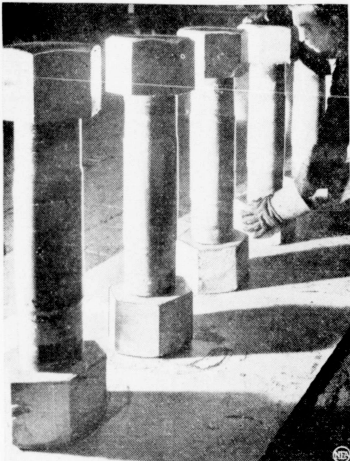
Striking photo is made as woman at East Pittsburgh Westinghouse works coats 315-pound stud bolts with protective compound. Bolts will join sections of a steel shaft of a giant generator.
