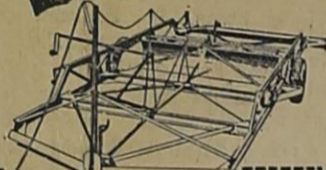
MODEL 25—Width 12'10", length 32', cutting blade length 9'3", depth 22", requiring 38 H.P. (drawbar).
