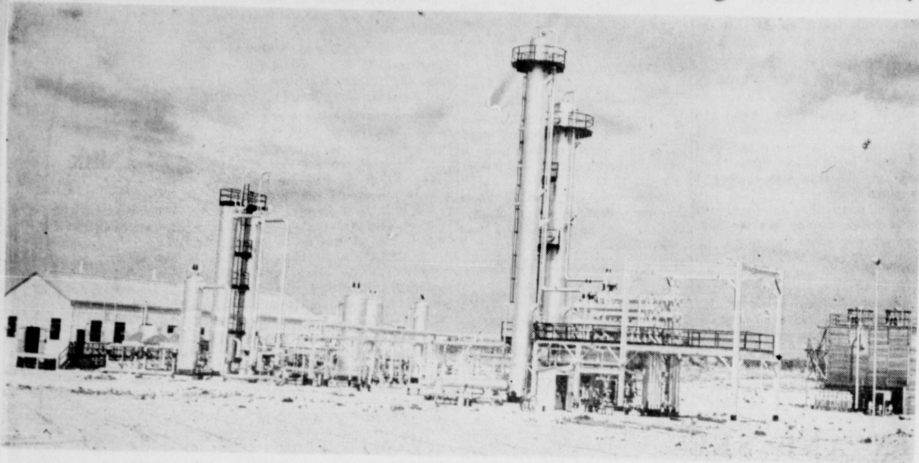
The Sun Oil Company Jameson Gas Plant at Silver, pictured above, built in the fall of 1948 and considerably enlarged in 1954, converts natural gas to propane, butane, and gasoline, up to 100,000 gallons per day, supplying the fuels tank trucks of dealers in this area, and putting the products also into pipe lines that cross
