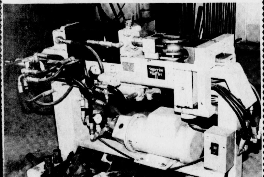
Pipe bending machine used to do all kinds of muffler & tail pipe work.
