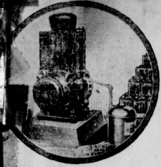
Delco-Light Model No. 320. For ranches, large farms and hotels. Ample light and power capacity.
