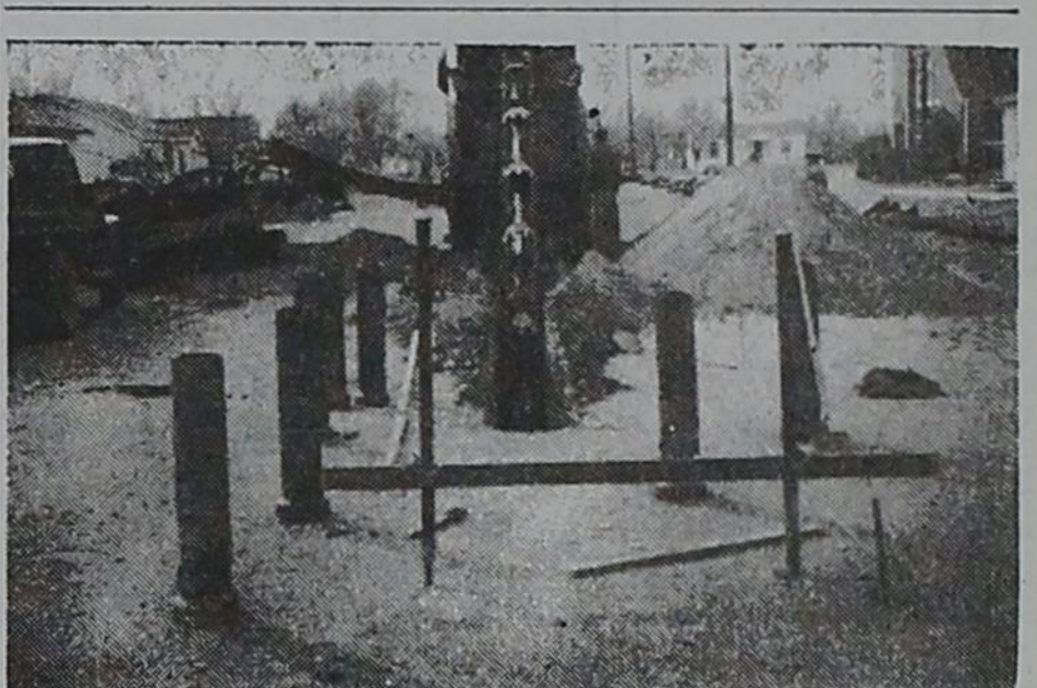
THE SEWER SYSTEM IS COMING and this big machine is doing a large part of the ditch digging. The machine, called a trencher, is pictured digging a 12 1/2 feet deep ditch. Some of the sewer lines will be as much as 16 feet deep. A total of 40,000 feet of ditches will be dug for the local sewer system.
