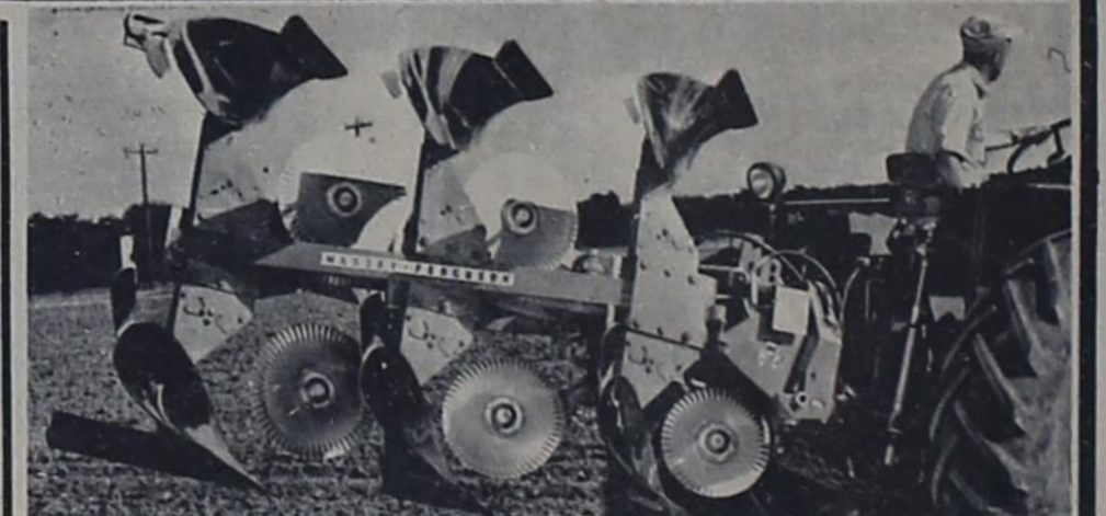
MF 57 Reversible Plow -- Mounted plow with hydraulic cylinder to reverse bottoms. Has 28 1/4" vertical trash clearance. Plow down to 16". Available in 3 or 4-furrow models with 16" or 18" bottoms. Ruggedness that has earned MF plows a reputation for good service and long life gives MF "two-ways" the same advantages. Steel frames are designed to give you a reserve of strength. 4-bottom model available.
