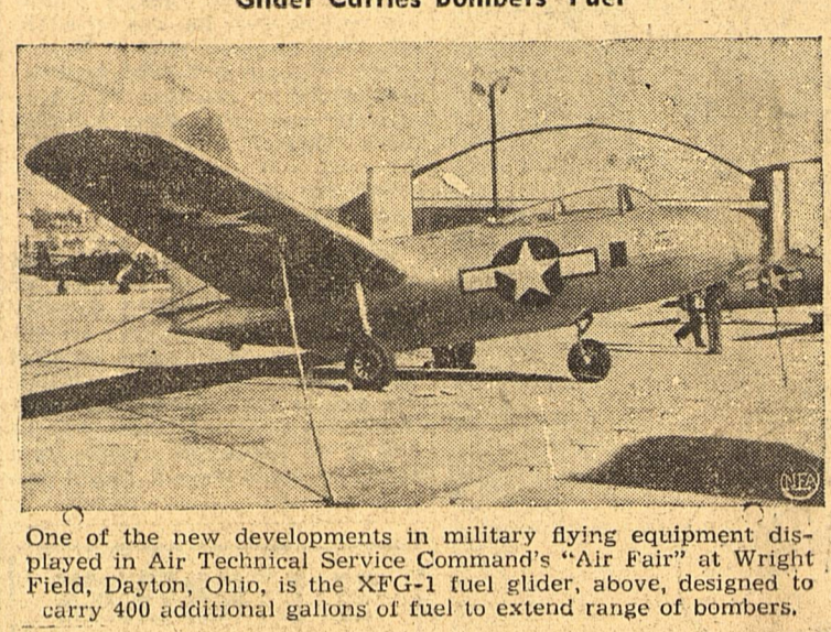
One of the new developments in military flying equipment displayed in Air Technical Service Command's 'Air Fair' at Wright Field, Dayton, Ohio, is the XFG-1 fuel glider, above, designed to carry 400 additional gallons of fuel to extend range of bombers.
