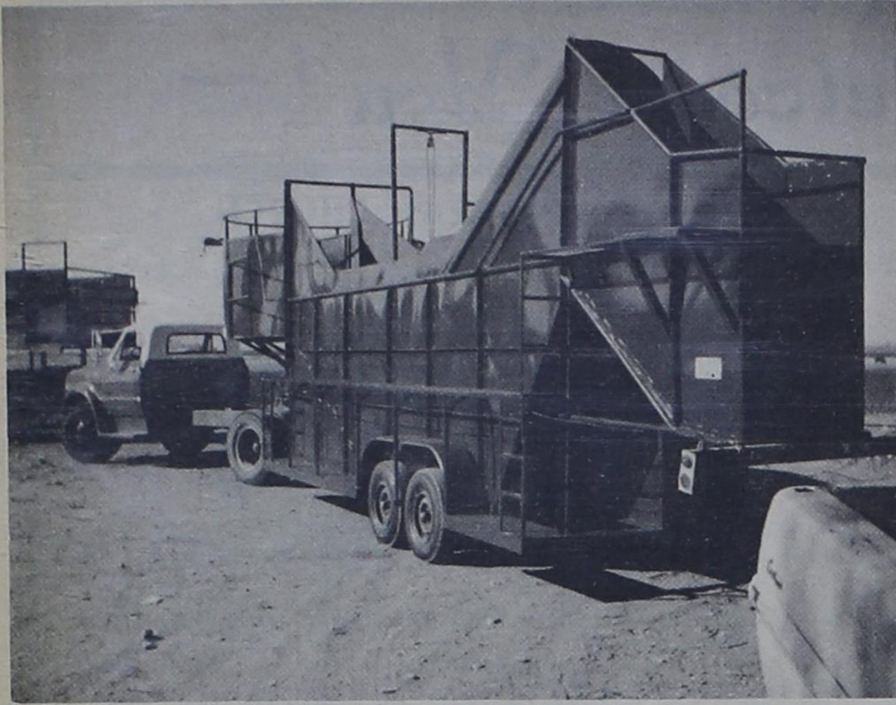
UNUSUAL DIPPING VAT --- The recent threat of scabies infection in cattle has increased the need for dipping in the area. This portable dipping vat was constructed by A. V. Warren at his place at Oklahoma Lane. A similar portable dipping vat is being operated in the area by Howard Looney. Only a loading chute is needed as an accessory to put the portable vats in operation. Such vats are unusual and attract much attention as they are moved from place to place.
