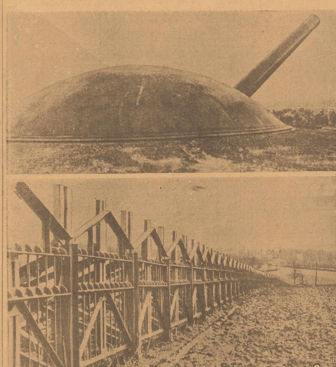
Belgium remembers 1914—when her old-style frontier forts were smashed by modern German artillery. Today her frontier with Germany is protected by a "Maginot" line similar to France's famed underground defenses. Above, a heavy gun rears from the top of a subterranean casement. The steel-reinforced anti-tank wall shown below runs over hill and dale for miles along Belgium's eastern border.
