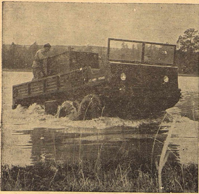
SWIMMING 2 1/2-TON TRUCK. Now undergoing rigorous tests, this 8800-pound vehicle can be air dropped and can travel cross country up to a speed of 55-miles per hour.
