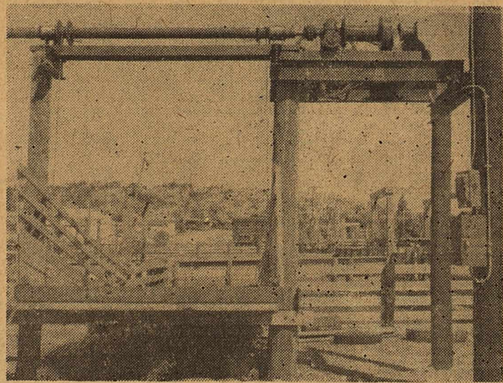
* The new automatic stock load controlled by the panel mounted on the light pole at the right of the picture. A lever on the panel raises or lowers the chute to any position required by the unloading truck.
