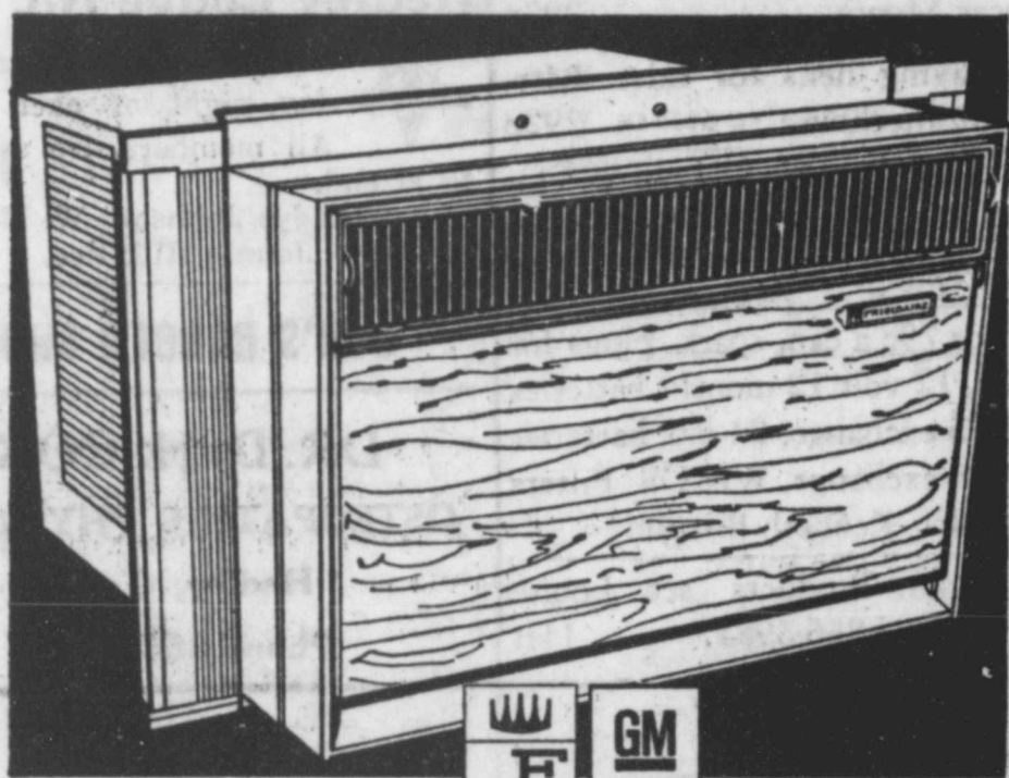
Model AEP-8ML—8,000 BTU/hr (NEMA) with optional walnut pattern front
