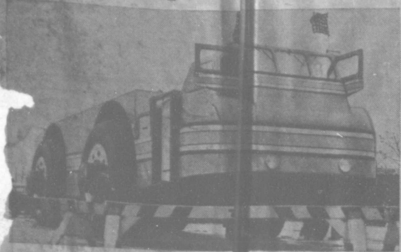
THIS SNOW CRUISER built by the Armour Institute of Technology will be used by Admiral Richard E. Byrd on his exploration trip through the Antarctic. Built at a cost of $100,000 the huge machine has a cruising speed of 24 miles per hour.
