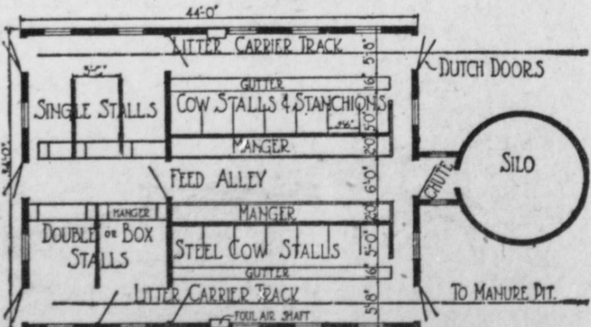
Ground Floor Plan of Horse and Cow Barn.
