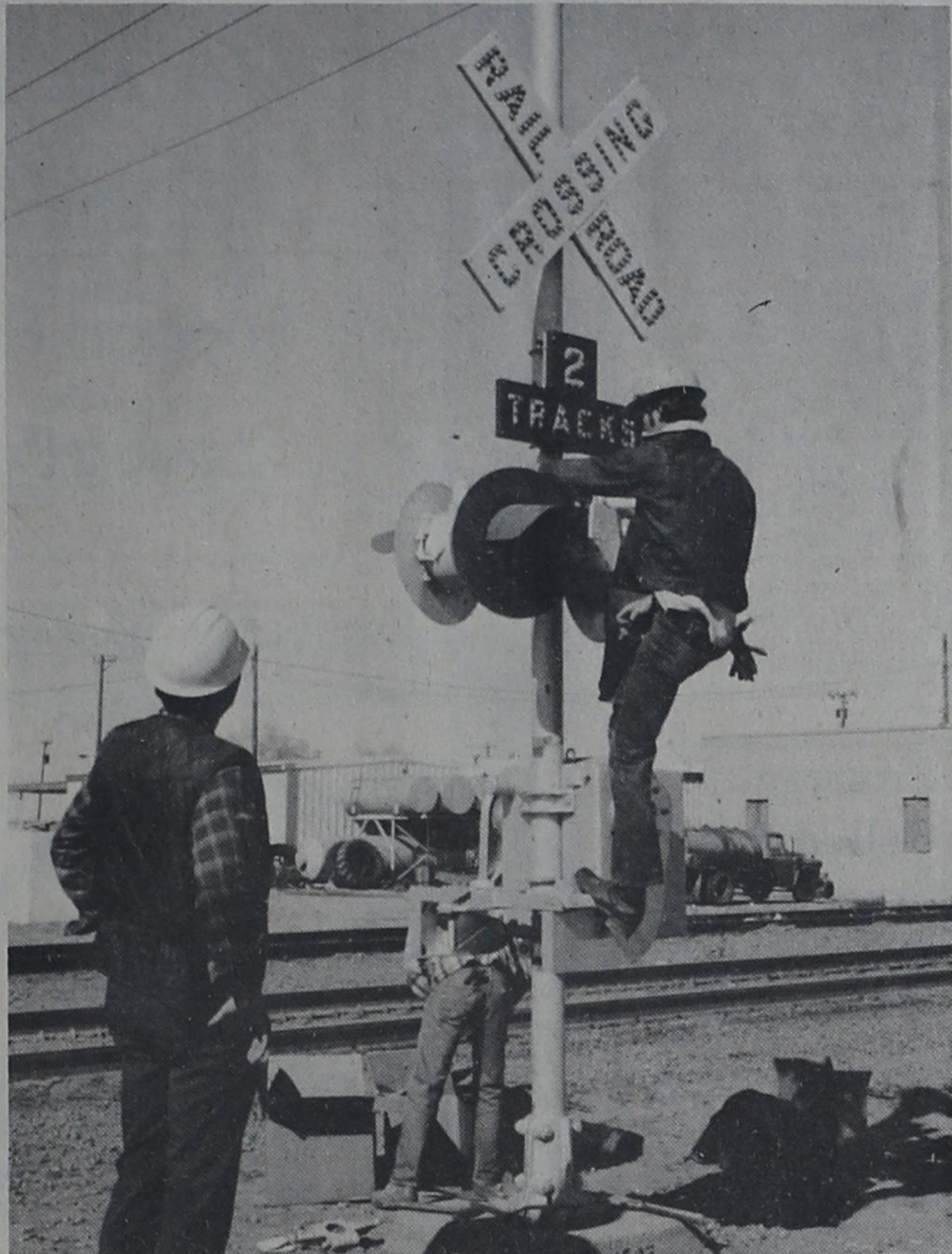
THIRD STREET GATES ...Preliminary work on railroad crossing gates on Third Street began Monday by a Santa Fe Railway Co. signal installation crew. C.O. McMillian, foreman of the crew, said the installation should be completed in two weeks barring any difficulties. Gates at the east Main crossing were put into operation in May of
