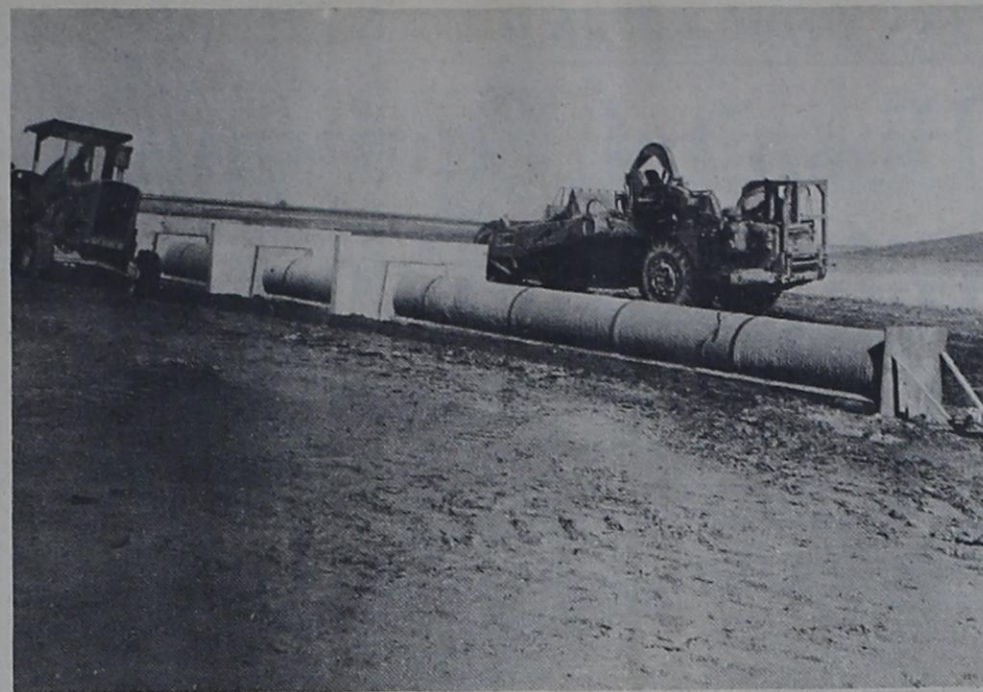
SPILLWAY GOES IN.... The three-foot pipe which make up the spillway at the Catfish Draw damsite north of Bovina is shown above, as the pipe was put in place recently. Officials of the Soil Conservation Service say the damsite is one-third completed.
