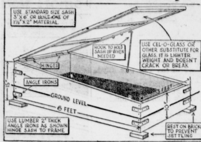
Working Drawing for Building Cold Frame.
