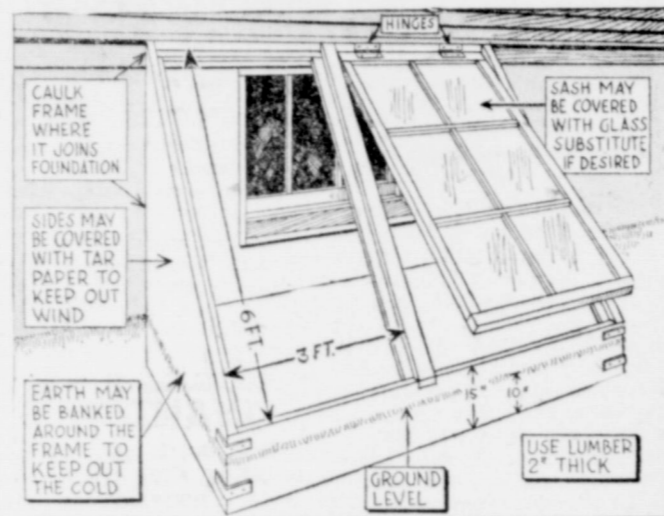
Working Drawing for Hotbed Outside Basement Window.
