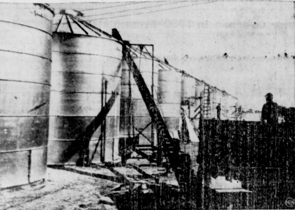
STORAGE FOR UNCLE SAM'S CORN —At Winterset, Iowa, the government is building storage bins to receive about 740,000 bushels of corn bought by the Commodity Credit Corporation. Eighty cylindrical steel bins, like those above, hold 3380 bushels each, 15 wooden bins will hold 60,000 bushels, and six Quonset-type buildings will hold another 60,000. As each storage unit is completed, it is filled with corn from the 1948 crop, freeing farmers' own bins for this year's big crop.
