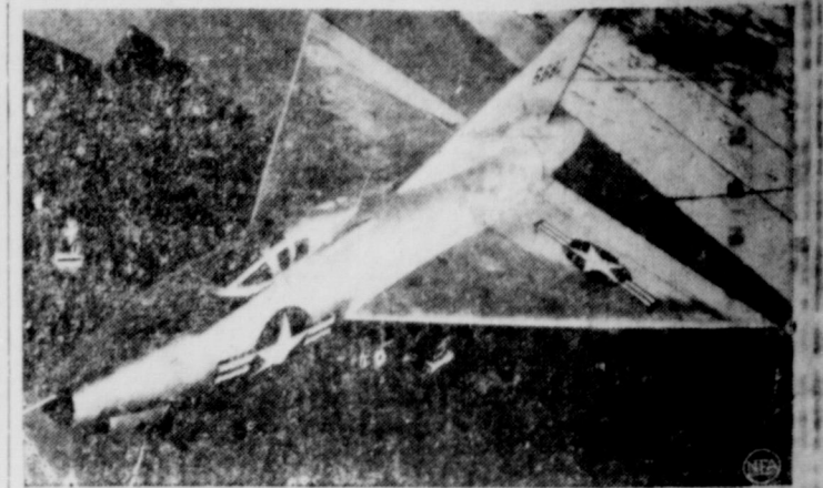
The Air Force's new research plane, Model 7002, prepares for a test flight at Muroc Air Force Base, Calif. The plane is equipped with a "Delta Wing," which is swept back at a 60-degree angle, compared to the 25-degree maximum on any other plane. The triangular wing has "elevons" in its trailing edges, eliminating the tail by combining the functions of aileron and elevator action. (U. S. Air Force photo from NEA-Acme.)
