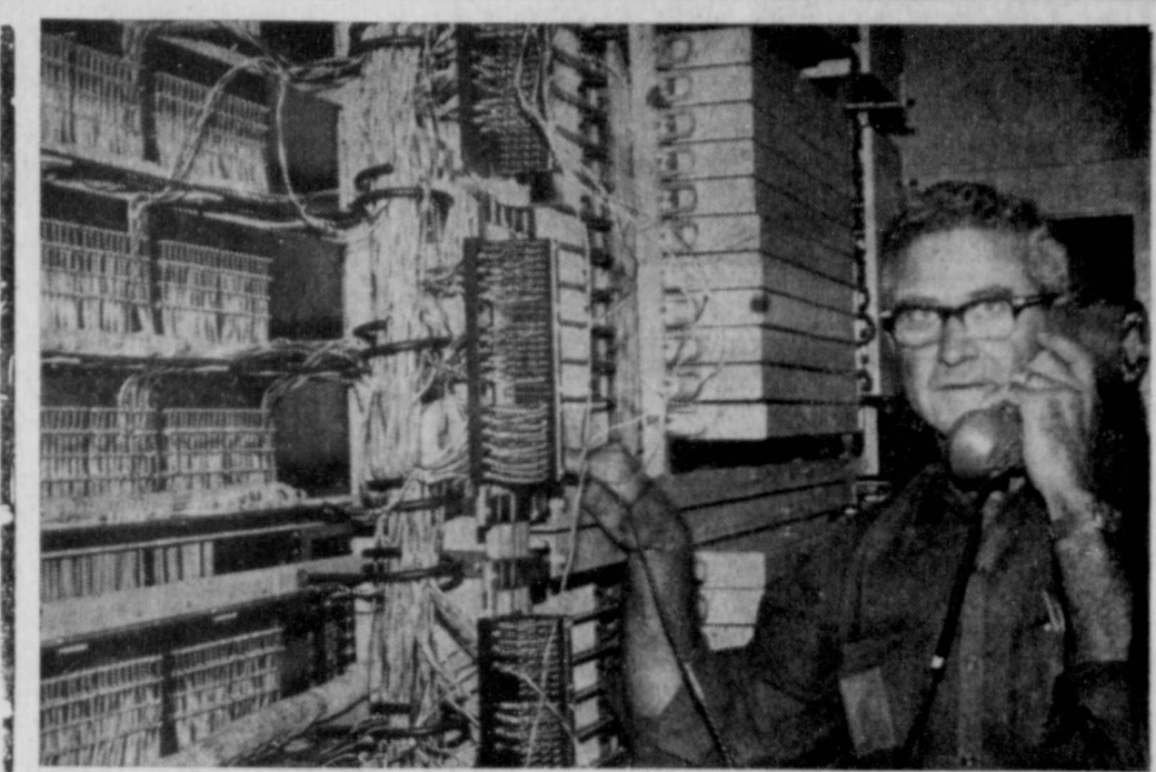
NEW TELEPHONE EQUIPMENT — Frank McClung, combinationman with General Telephone Company here, is shown testing some of the new central office equipment which was placed into use here early Sunday. Goldthwaite is one of seven central Texas communities that have access to equipment, making Expanded Direct Distance Dialing possible.
