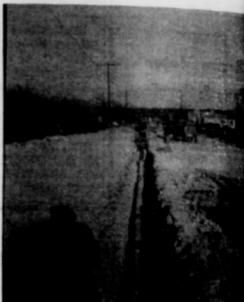
Placing Pipe in Ditch on West Sixth Street leaving the City and moving toward Water Treatment Plant.
