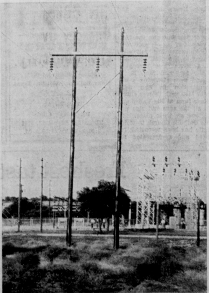
NEW STRUCTURE —Here is an average structure, and new 69,000 volt capacity line with conductor, that has been constructed by Lower Colorado River Authority from San Saba to Goldthwaite. The project consists of San Saba and Goldthwaite substations with 19 miles of line costing over $300,000. The new line has a carrying capacity of approximately 10 times the old line. During construction period of this project the City of Goldthwaite built a heavy added circuit from the substation to town. This provides the electric distribution system of the city five times the capacity of the old line. Both the old and new lines into town are now being used by the city.
