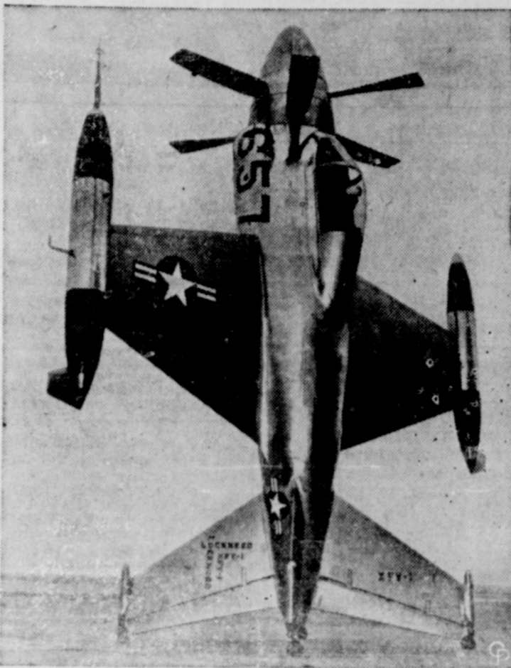
A SENSATIONAL departure from conventional take-offs is achieved by the Navy's new XFV-1 fighter plane, shown resting on its tail in Burbank, California. The unusual craft is designed to land and shoot upward from the ground in this position. It is powered by turbo-prop engines, with counter-rotating propellers. (International Soundphoto)
