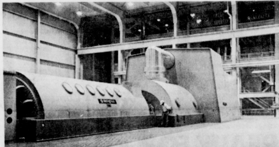
THE ELECTRIC GENERATOR at Southwestern Public Service Company's new Harrington Station is rated at 356,700 kilowatts, the equivalent of 478,000 horsepower. The turbine rotates at 3600 rpm and its speed is controlled so that it is constant, within one revolution per day. This amazing accuracy keeps electric clocks on time and is used by industry for precision control of production operations. The generator output is 22,000 volts which is then stepped up by a transformer to 230,000 volts for more efficient power transmission.
