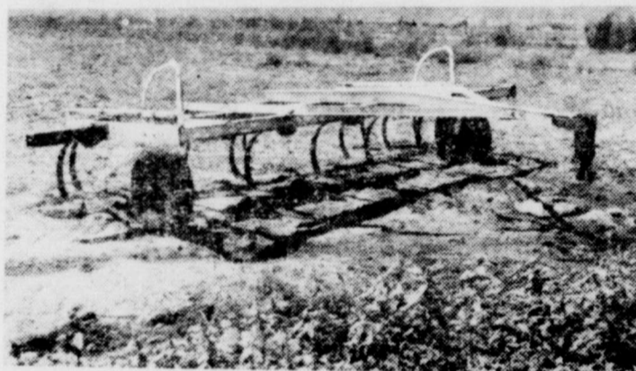
This photo shows a chisel plow equipped with 14-inch sweeps. This is probably the most common implement used in Foard County for stubble mulch farming.
