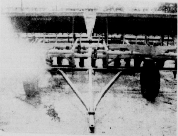
Pictured above is a deep furrow drill. These drills are especially designed for stubble mulch farming. This is one of the pieces of equipment to be demonstrated.
