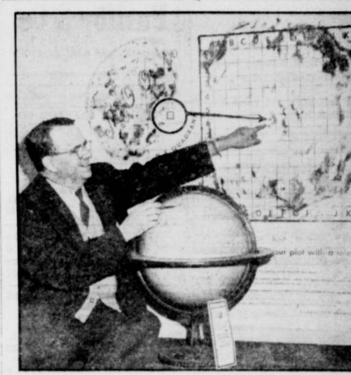
LUNAR LOTS FOR SALE —Robert R. Coles of Glen Cove, N.Y., points to "allotment" on part of the moon's Crater of Copernicus. Area shown is an enlargement of circled area on telescopic picture of moon, at left. A former chairman of New York City's Hayden Planetarium, Coles has incorporated "The Interplanetary Development Corporation." He hopes to sell moonscapes at one dollar an acre. Buyer supplies his own transportation if he wants to "moonstead" his land.
