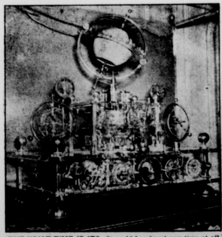
BUT WHAT TIME IS IT? —It could be almost any time at all, if you had this clock, and the knowledge necessary to interpret its indications. Displayed in Paris, France, by inventor F. J. Senec, the instrument is set to give, for 100 years, the following information: Day, date, month and year; occurrence of Easter; phases of the moon, sidereal and mean solar time; predictions of approaching lunar and solar eclipses.
