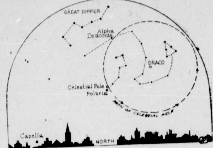
Constellations in the northern sky at 9 p. m. on June 1.
