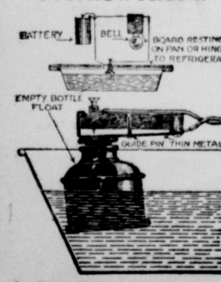
An alarm to be placed in the drip pan of a refrigerator to sound when the pan is full, may be made as shown above.
