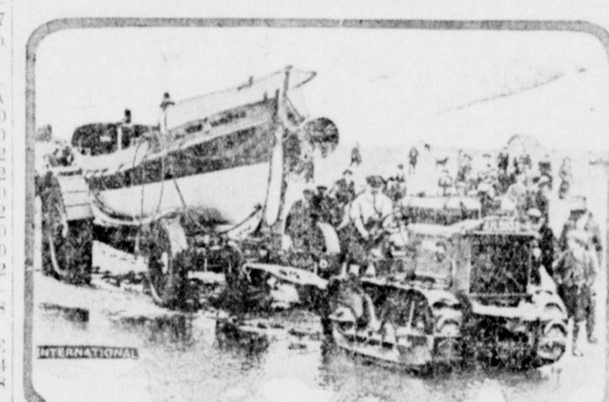
A specially constructed caterpillar for launching lifeboats was successfully tested recently at Humberston, England. The tractor draws the lifeboat, on a specially built carriage, to the beach and then, reversing, pushes it into the sea beyond the breakers, eliminating the chance of the boat overturning.
