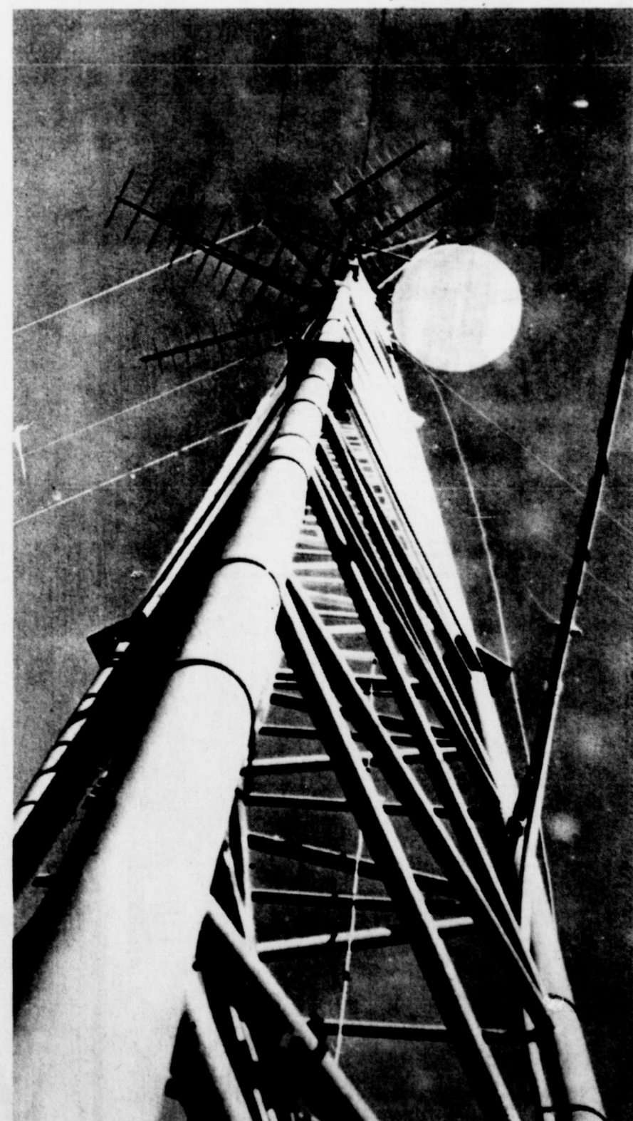
TALL RECEIVER—This is a view from the ground of the receiving antenna tower which will gather television signals for the cable television project now under construction in Winters. This tower is about 150
