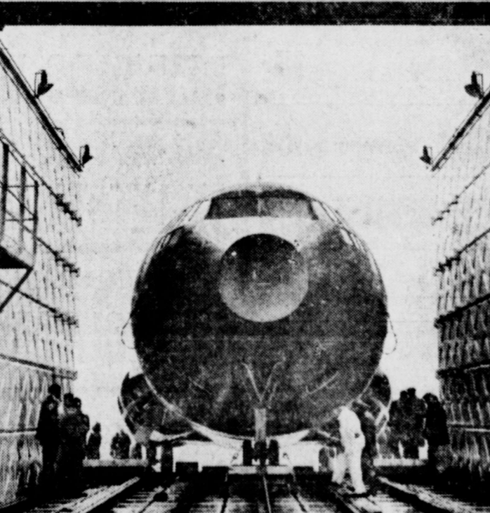
TORTURE TEST —Workers roll the nose of a transport into its "torture" chamber. The test about to result will subject the plane to simulated loads and strains likely to be encountered in a normal service life of 10 years. Water is pumped through the fuselage under extreme pressure in cycles, and tension jacks flex the wings and fuselage at the same time. Test is taking place in Belfast, Ireland.
