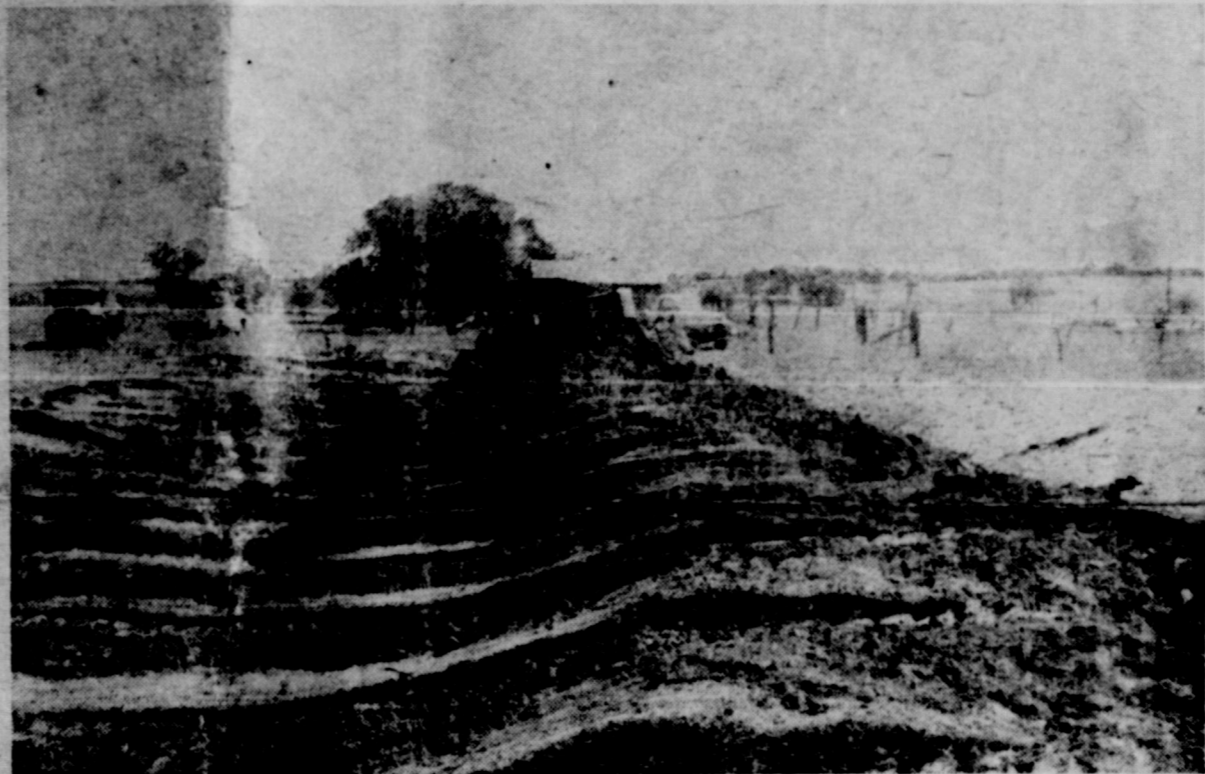
This photo shows the second trip with the dozer. The next step is the final grading of the terrace channel and ridge by running the dozer lengthwise of the terrace.
