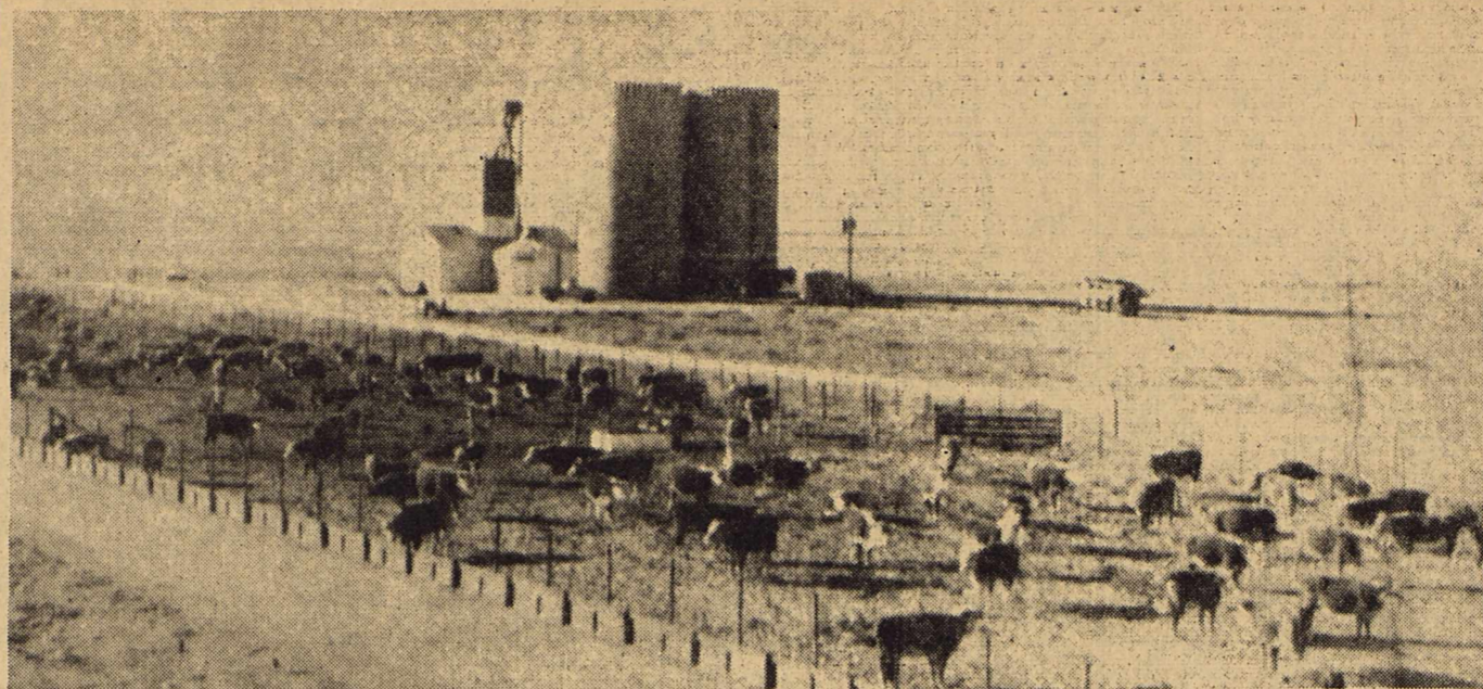
Over all view OF THE BENNETT cattle feeding plant, showing the four separate pens with a capacity of 800 head for each feeding period, the batch mixing mill. In the background can be seen two 60-foot high upright silos and a portion of the initial herd on a 120 day feeding program. In the background can be seen two 60-foot high upright silos and the batch mixing mill. PRESSphoto
