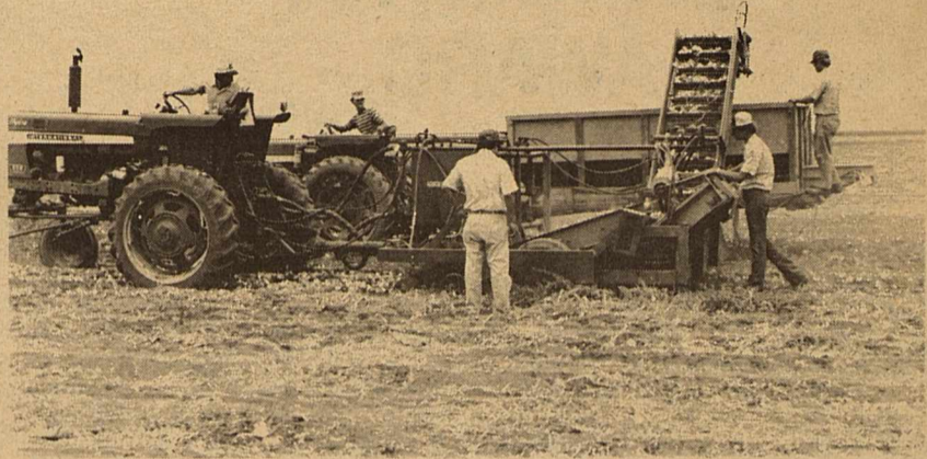
THE TEXAS AGRICULTURAL EXPERIMENT STATION'S prototype automatic onion picking machine was being tested at Evergreen Farms.
