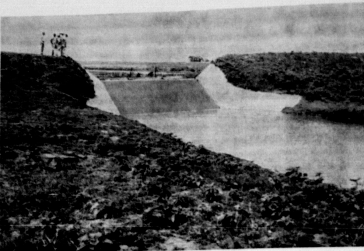
GRADE STABILIZATION STRUCTURE —Shown above is a grade stabilization structure of concrete and rock masonry which was cost-shared under the Great Plains Conservation Program in 1959. This structure is located on the Ed Hutcherson farm on U. S. Highway 287 8 miles southeast of Memphis. (See story on Page Five)
