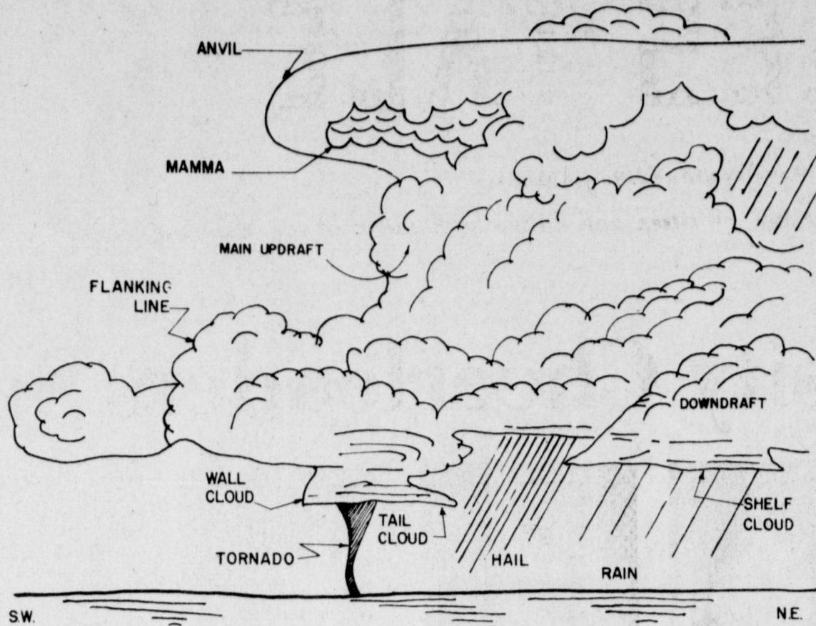
TYPICAL TORNADO-PRODUCING CLOUD... The form of the usual tornado-producing cloud is anvil-shaped at its crest with a rougher overshooting top at the dome. Mamma, which appear to be balloon-shaped formations, may drop from the anvil shape. At ground-level the common appearance is rain falling from a shelf cloud, usually in the northeastern portion of the parent cloud. Southwest of this there will be a wall cloud, sometimes with a horizontal tail cloud at the forward or northeast lower portion of it. This tail cloud is not the tornado. The tornado itself forms typically at the southwest lower edge of this wall cloud. Behind the tornado there is not likely to be rain, but, instead, a precipitation-free cloud base. [Drawing courtesy Texas Tech University Institute for Disaster Research]
