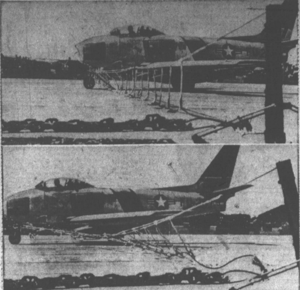
NET RESULTS ARE GOOD—A plane-and-pilot saver might well be the name for this device which has been developed by the Far East Air Force's 6400th Maintenance group. The net stops fast-landing damaged jet aircraft and enables them to land on small emergency strips near the fighting front. In the top photo, the nose wheel of the plane touches a line which triggers the main arresting gear (bottom photo) which engages the main landing gear and brings the plane to an easy halt. The net, similar to those used on aircraft carriers, cost $14,000 and has already saved 10 jet planes worth $240,000 each and possibly the lives of 10 airmen
