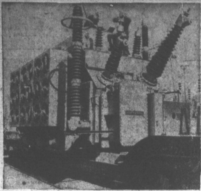
PORTABLE VOLT JOLTER —Resembling an artillery piece from outer space, this 340,000-pound transformer is the largest portable transformer in the United States. Built for the Bonneville Power Administration, the transformer "steps down" electricity from 220,000 volts to 115,000 volts. Shown here in Goshen, Ore., it is mounted on a 175-ton railroad flat car.
