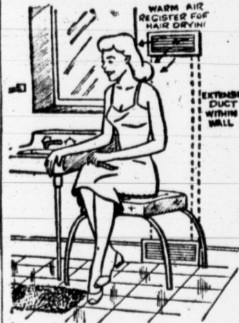
BUILT-IN hair dryer can be provided by extending warm air duct head height for woman seated.
