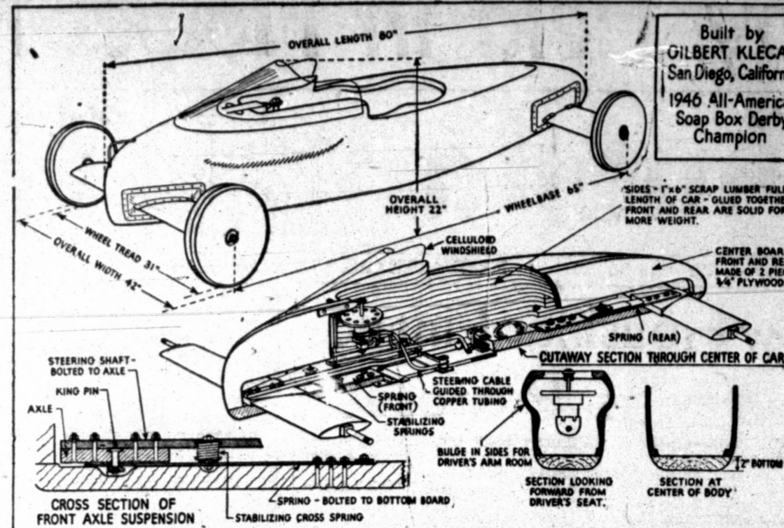
The prize-winning All-American Soap Box Derby racer of 1946, built by Gilbert Klecan, after the race, may give 1947 contestants some ideas on how to improve their own car designs.
