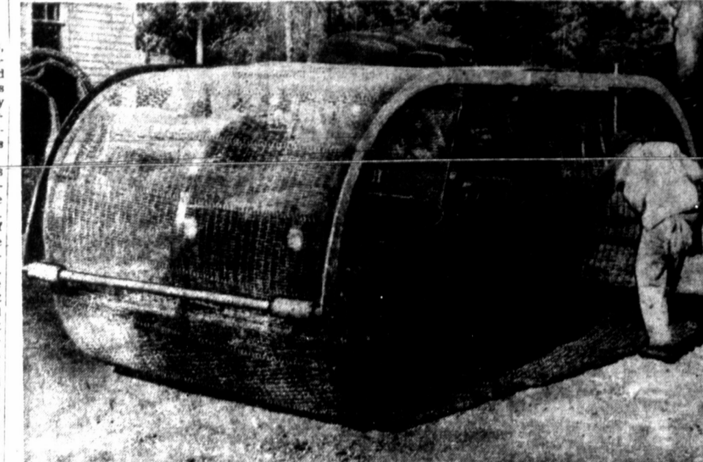
Marines at Quantico, Va., have developed this "squirrel cage" for their jeeps. A belt of road matting runs under the wheels and then back over the top, providing a continuous portable road surface wherever the jeep goes. The vehicle can drive through swamps, bogs, soft beaches and underbrush.
