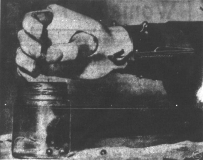
This is an experimental model of a new mechanical hand, which has joints like a human hand. Being tested at the Emergency Limb Center, in London, it picks up a ball bearing between fingers and thumb. It has also successfully picked up cigarettes, pins and other small objects.
