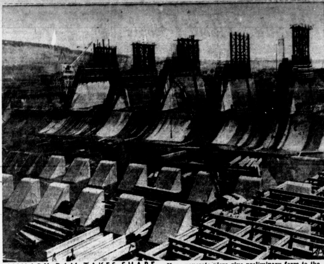
M'NARY DAM TAKES SHAPE —Huge concrete piers give preliminary form to the spillway section of the $227,000,000 McNary Dam on the Columbia River between Oregon and Washington, scheduled to be finished in 1953. It is named for Oregon's late Senator, Charles L. McNary.
