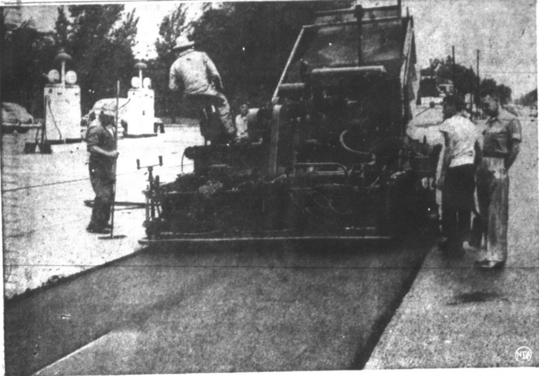
HERE'S A ROAD WITH EXTRA BOUNCE —Cars should really bounce along this strip of roadway in Columbus, O. It's one of two streets where the Ohio Highway Department is laying a 300-foot experimental patch of rubberized pavement. The sample strips, 12 feet wide, will each include more than 400 pounds of rubber. The rubber roads will be studied as to durability and non-skid qualities. The project is expensive, and it will take years of testing to determine whether rubber roads are practicable.
