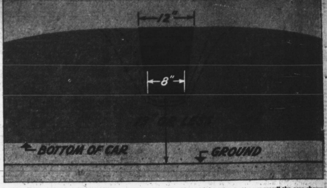
This diagram illustrates the size of the cockpit opening. The sides must be cut away to remove all the area shown in black in this drawing. The opening may be wider or deeper or of different shape, as suggested by the dotted lines. The 13-inch measurement from the ground must be taken when the car is empty.
