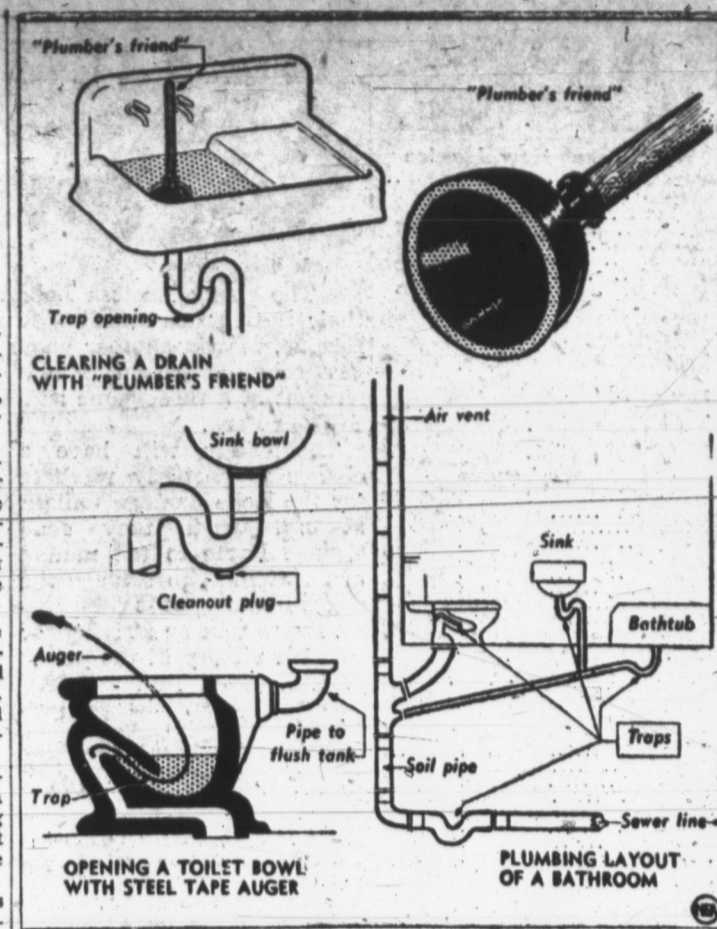
These diagrams should help you to open up clogged drain pipes.
