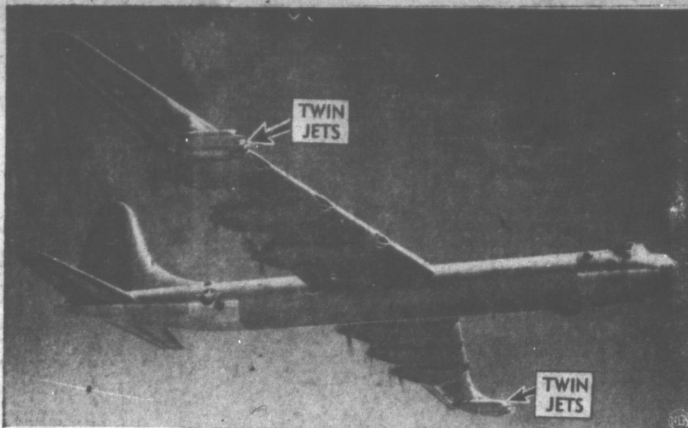
JETS BOOST POWER OF B-36—Heading for the wild blue in its first high-altitude flight over San Diego, Calif., is the Convair B36-D, a "souped-up" version of the world's biggest bomber. Four jet engines, mounted in pairs under the outer wing edges, add to the bomber's six piston engines to give it a total of over 40,000 horsepower for take-off and enabling the ship to travel 435 miles per hour and reach altitudes above 45,000 feet. (Department of Defense photo from NEA-Acme Telephoto.)
